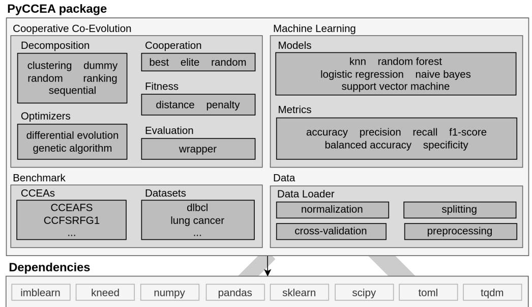
Figure 1: An overview of the PyCCEA package, its underlying Python resources. We emphasize that this figure does not show all modules of PyCCEA. .
