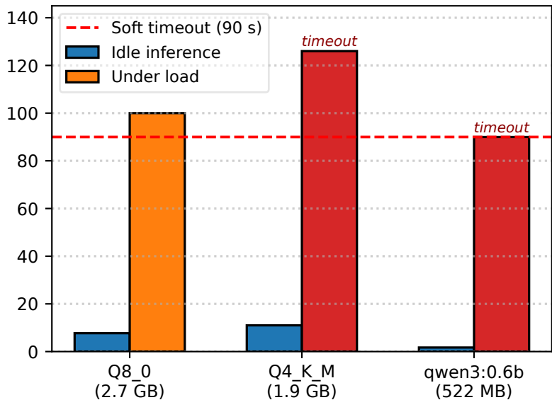
Inference Time (s)
