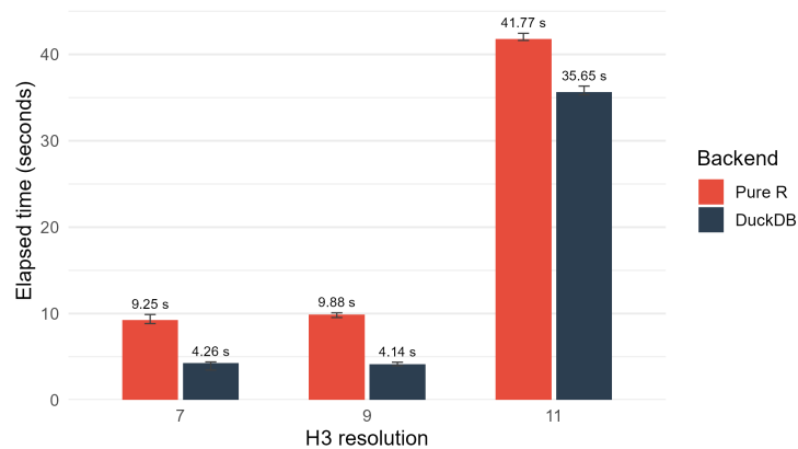
Figure 6: Elapsed time (s) for cnefe_counts() on Curitiba-PR, by H3 resolution.
