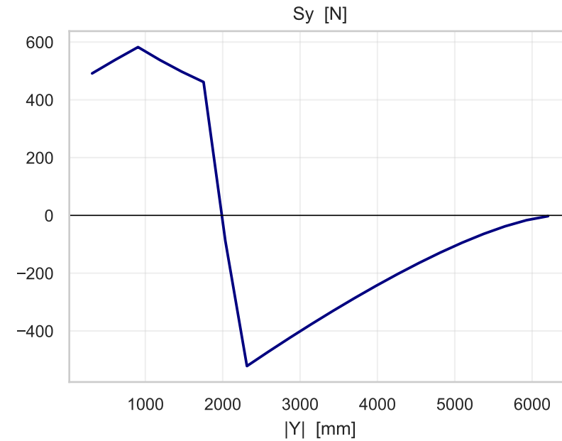
Best-design internal force / moment diagrams (load case 0)
