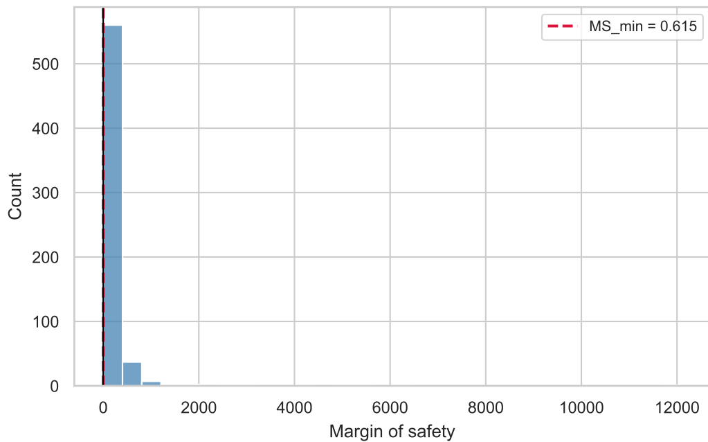
Tsai-Wu margins of safety
