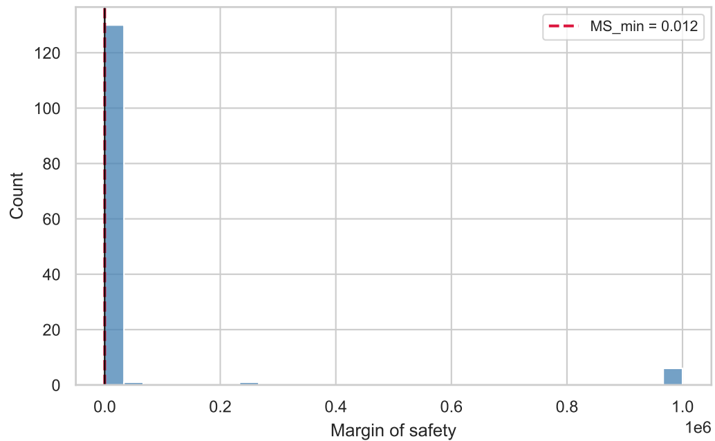
Displacement margins of safety
