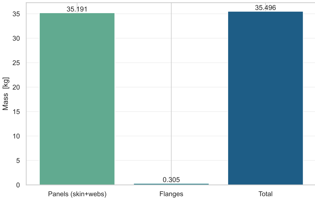
Best-design structural mass breakdown
