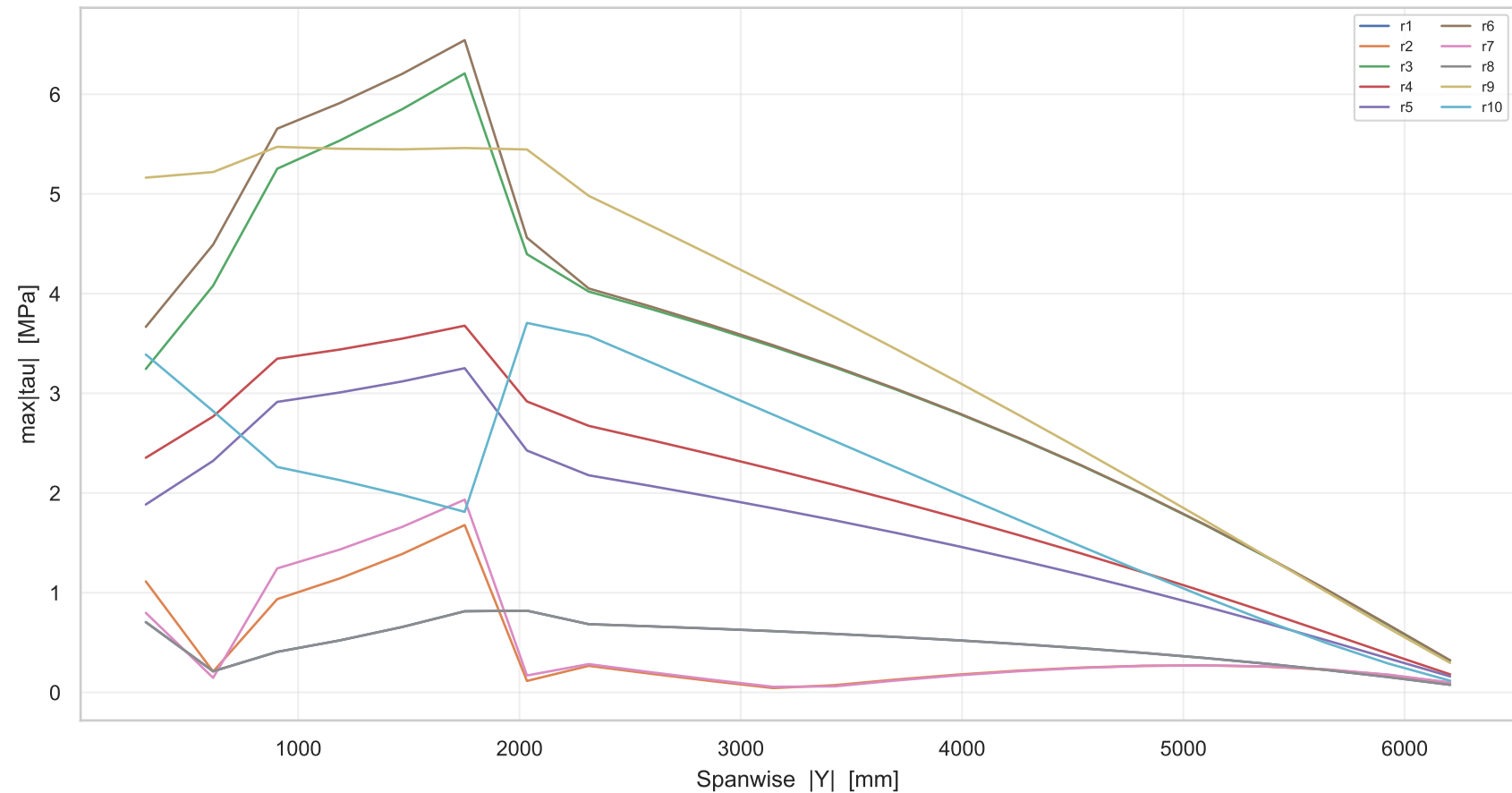
Per-panel shear stress along span (load case 0)
