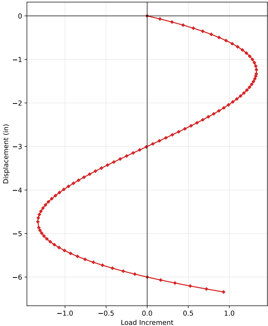
Fig. 15: 'Four-member truss' (GDC)
