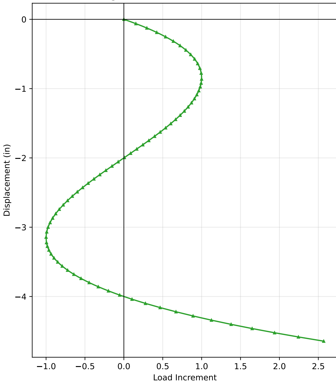
Fig. 6: 'Two-member truss' (GDC)
