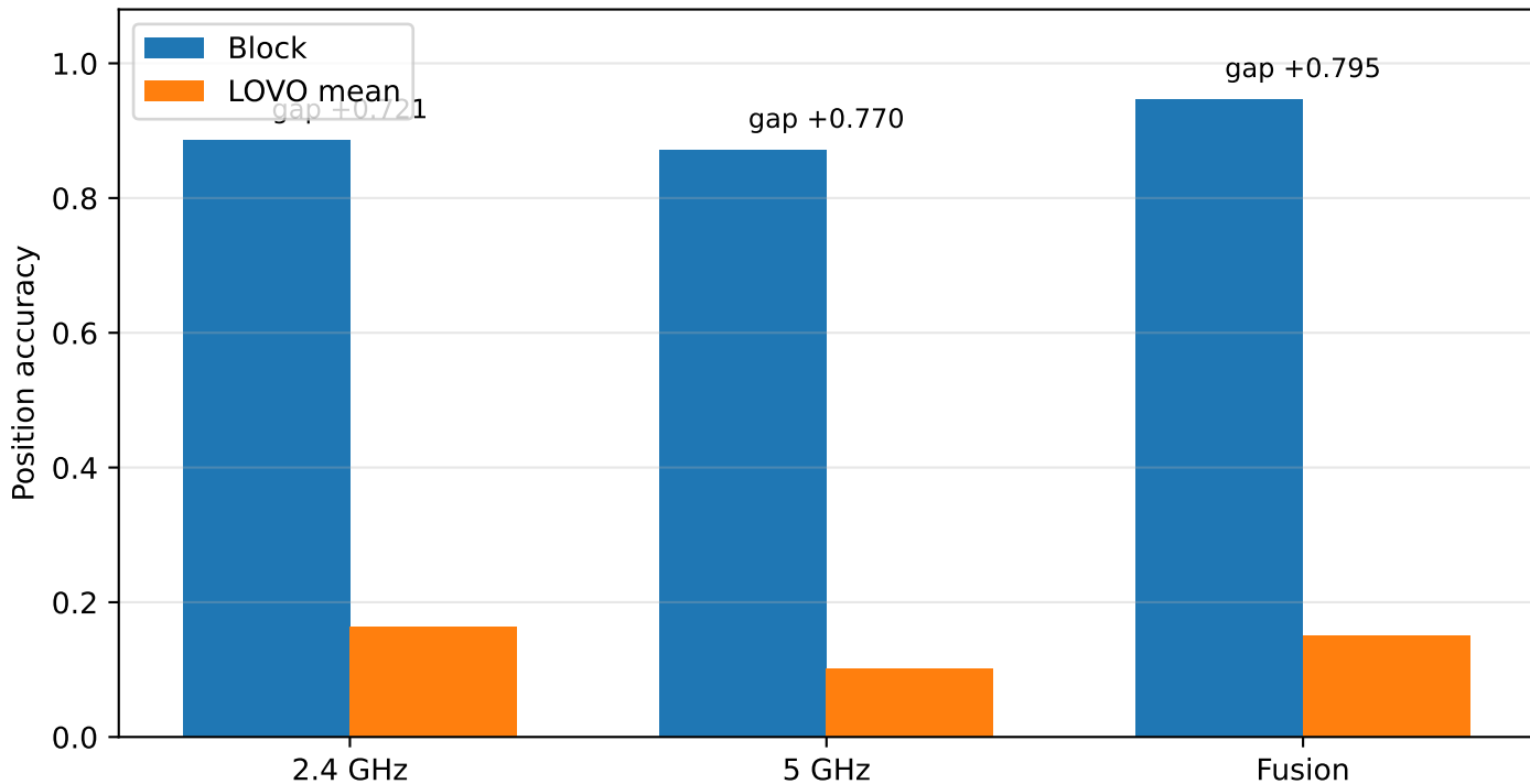
Block vs LOVO cross-user generalization cost - RF
