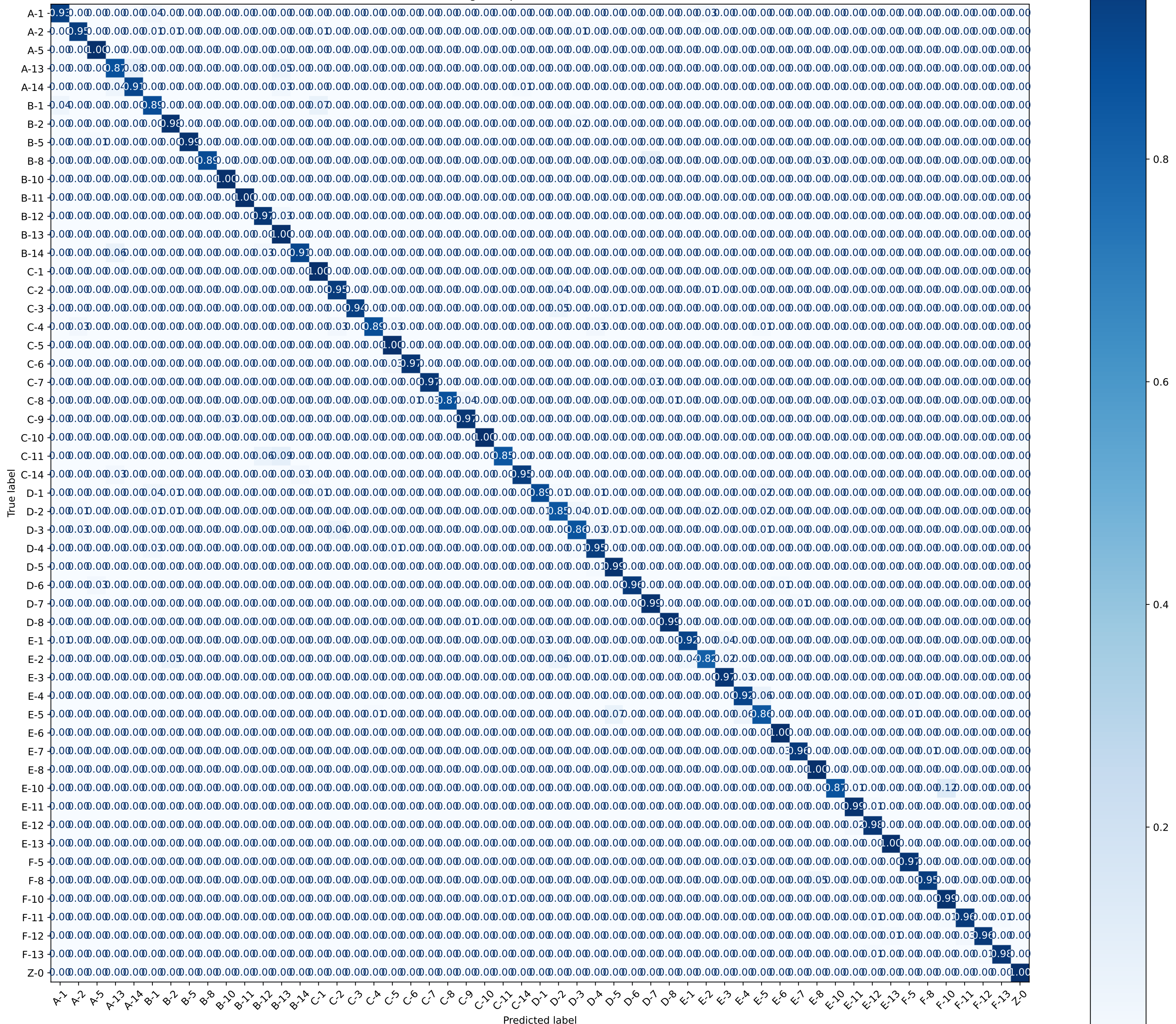
Predicted label
