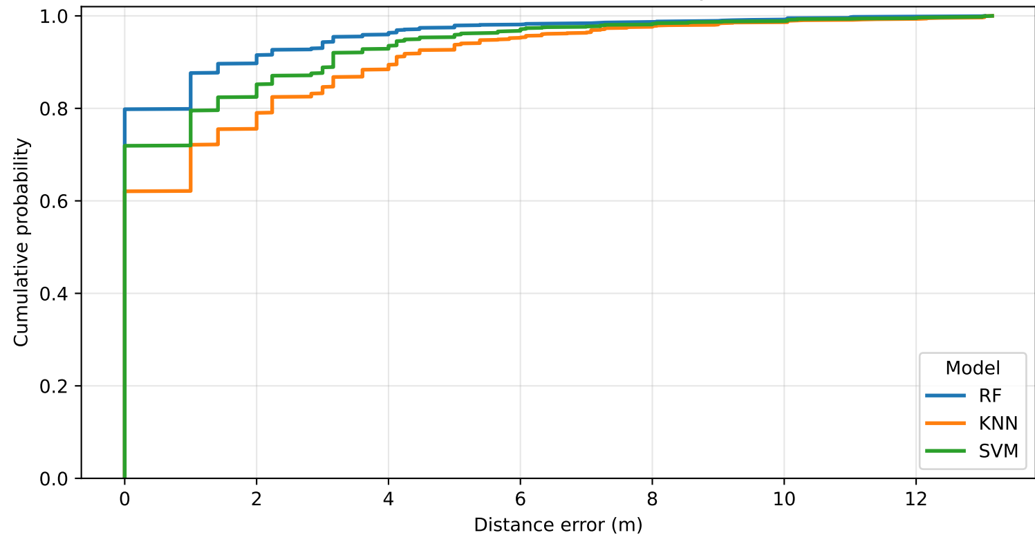
2.4 GHz - localization error CDF by model
