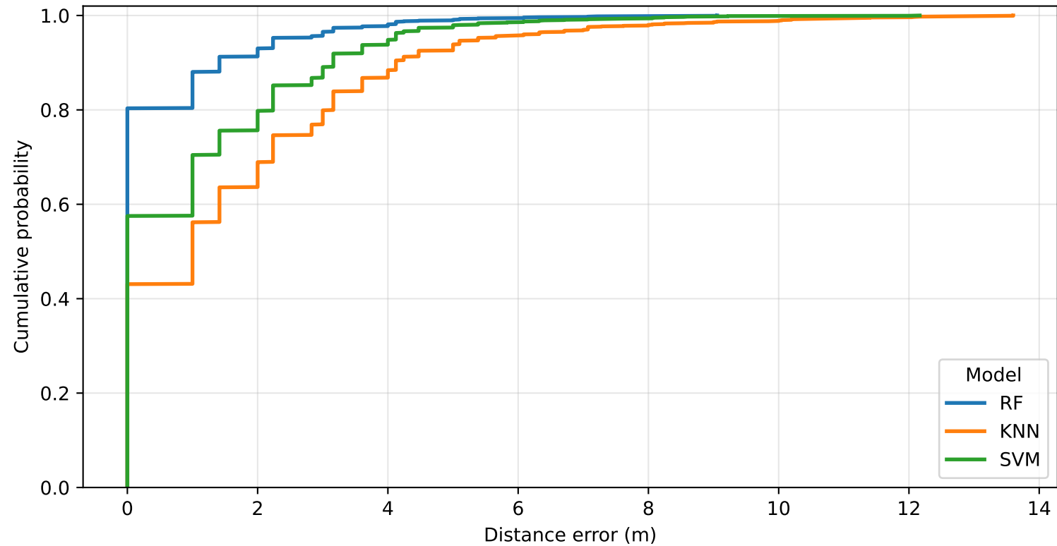
5 GHz - localization error CDF by model
