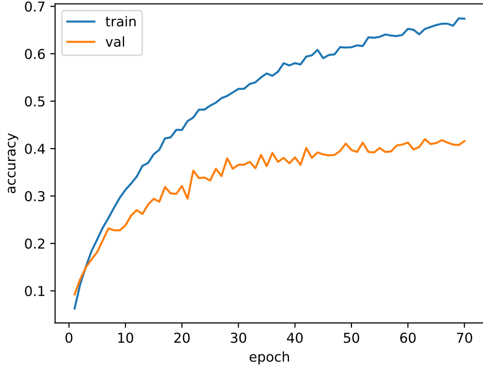
CNN - 5 GHz - cross_session accuracy
