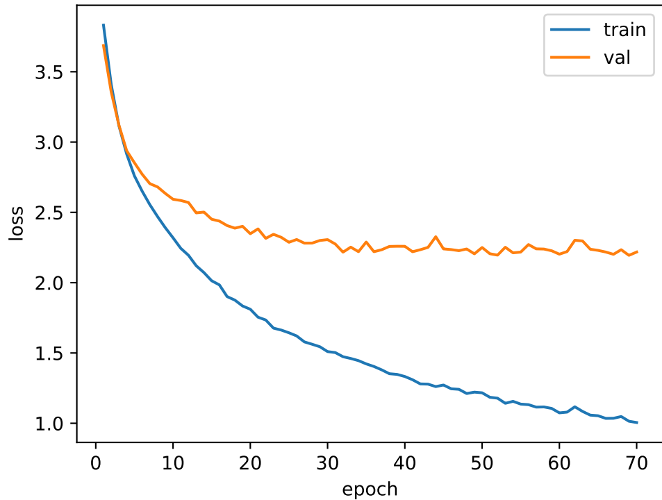
CNN - 5 GHz - cross_session loss
