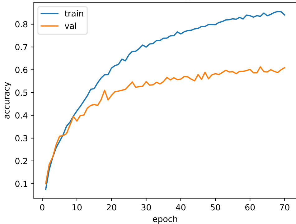
CNN_room - Fusion - cross_session accuracy
