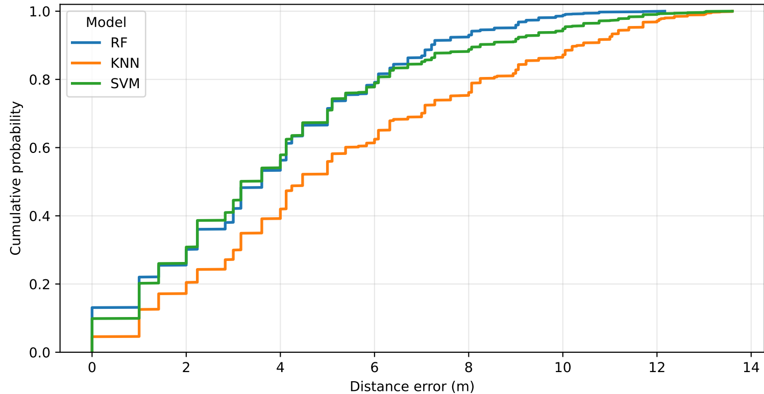
5 GHz - localization error CDF by model
