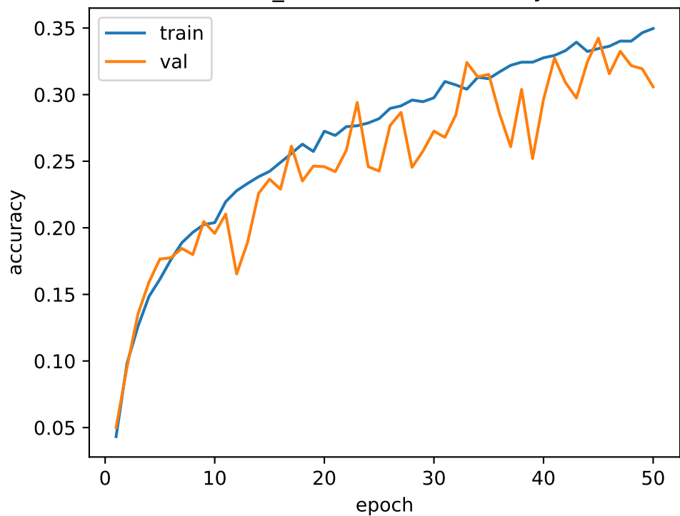
CNN_small - 5 GHz accuracy
