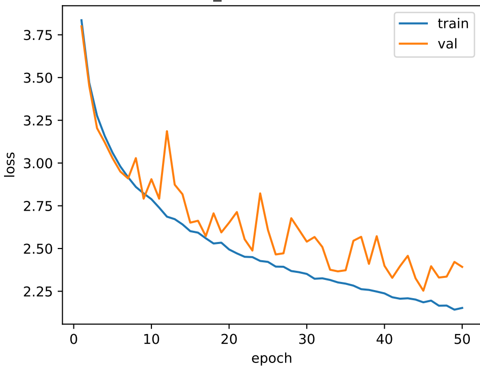
CNN_small - 5 GHz loss
