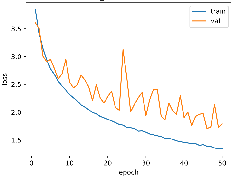
CNN_small - Fusion loss
