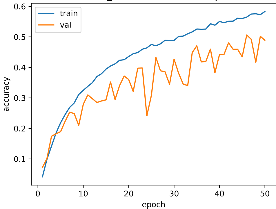
CNN_small - Fusion accuracy
