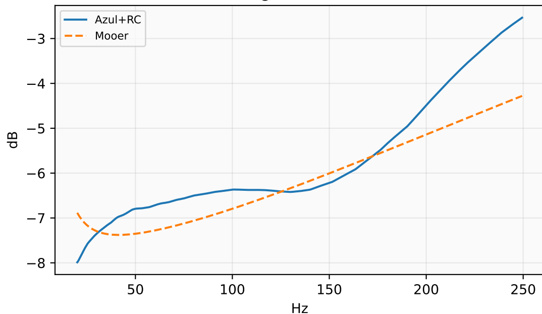
Zoom graves ≤250 Hz
