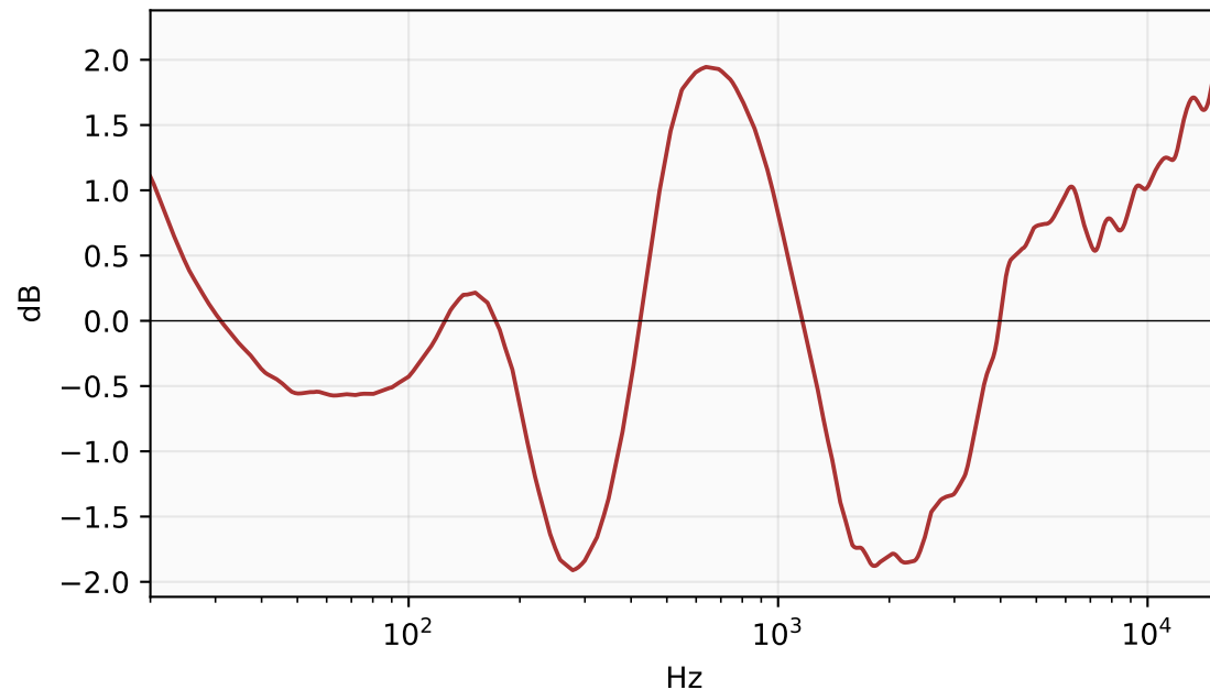
Error (Mooer – Azul–RC)
