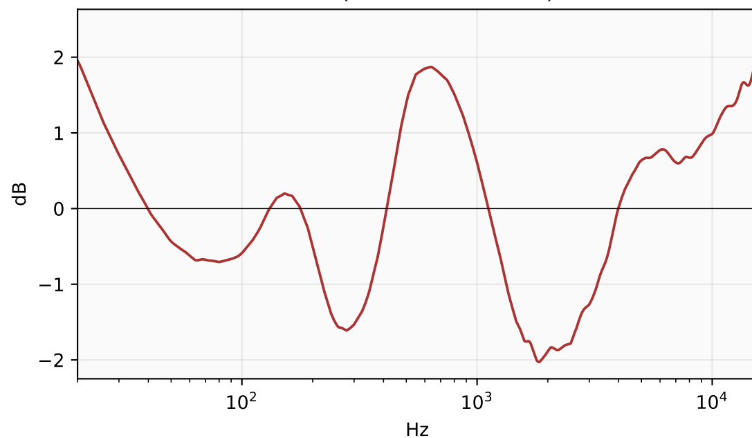
Error (Mooer – Azul–RC)
