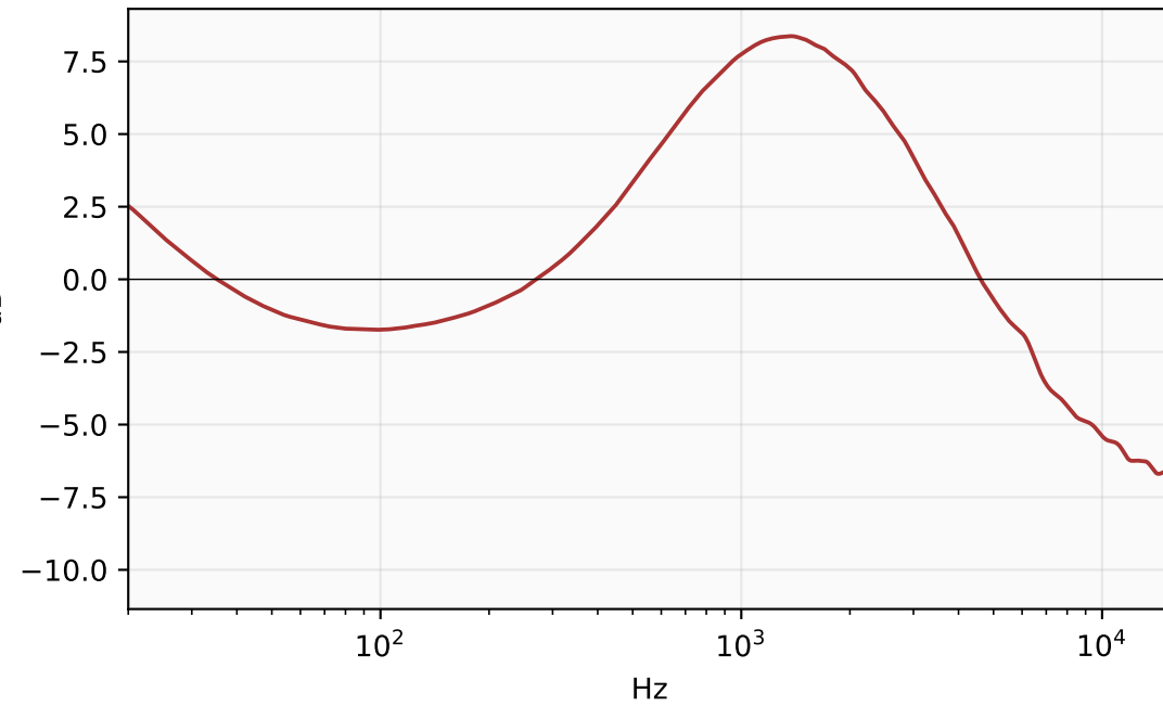
Error (Mooer – target)
