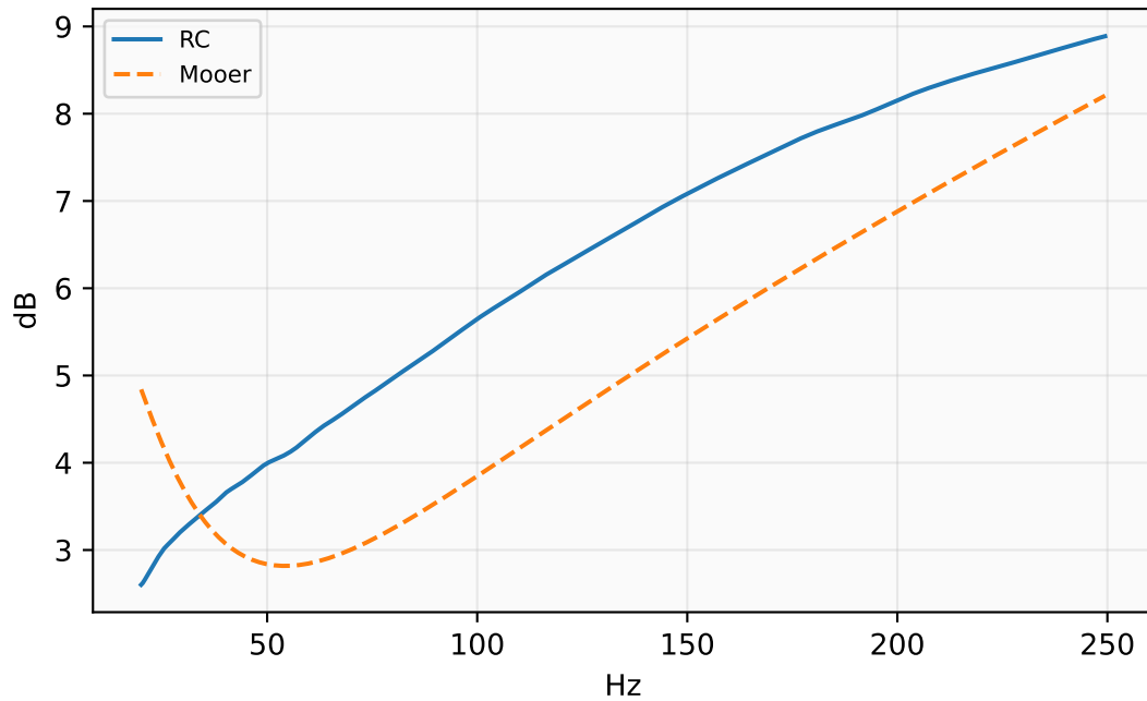
Zoom graves ≤250 Hz
