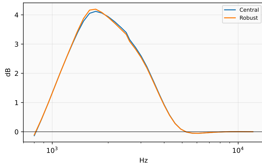
Zoom 0.8-12 kHz
