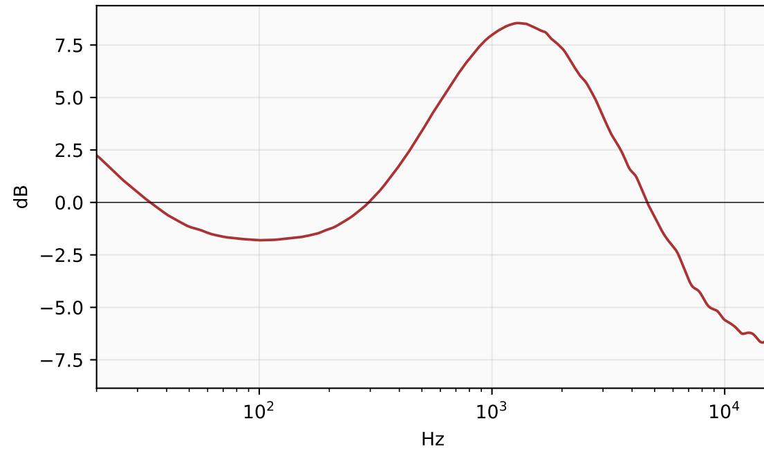
Error (Mooer – target)
