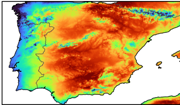
ConvCNP (topography-only)
