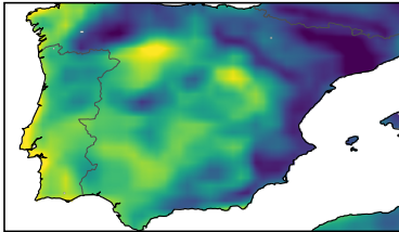
ERA5 bilinear interpolation
