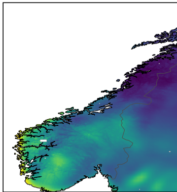
ConvCNP (topography-only)
