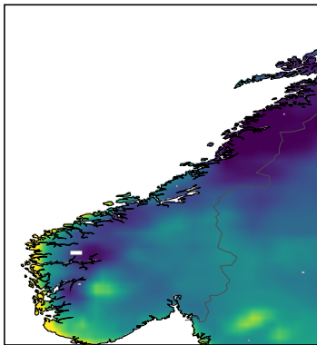
ERA5 bilinear interpolation
