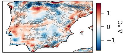
\Delta = \text{TESSERA} - \text{topography-only} (mean +0.22 ^{\circ}\text{C} removed)
