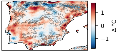
\Delta = \text{TESSERA} - \text{topography-only}
