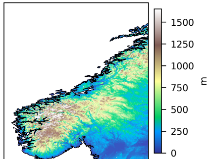
terrain elevation
