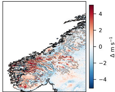
\Delta = \text{TESSERA} - \text{topography-only} (mean +0.96 \text{ m s}^{-1} removed)
