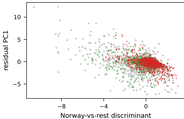
TESSERA lat16 embedding reachable 96%, AUC 0.96
