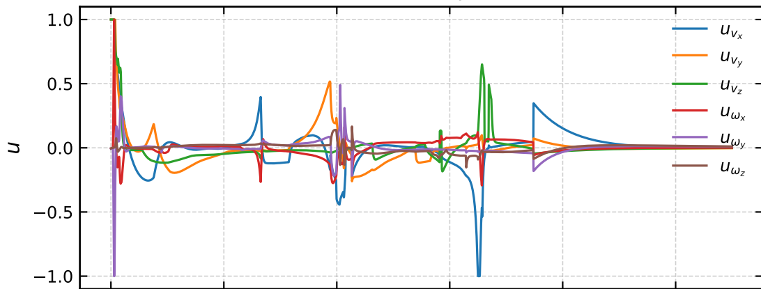
System Twist
