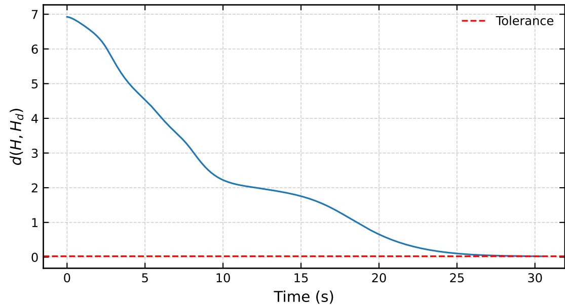
Pose Error
