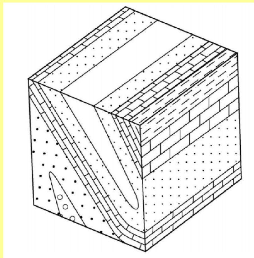
SINCLINAL
