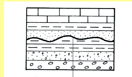
Discontinuitat
