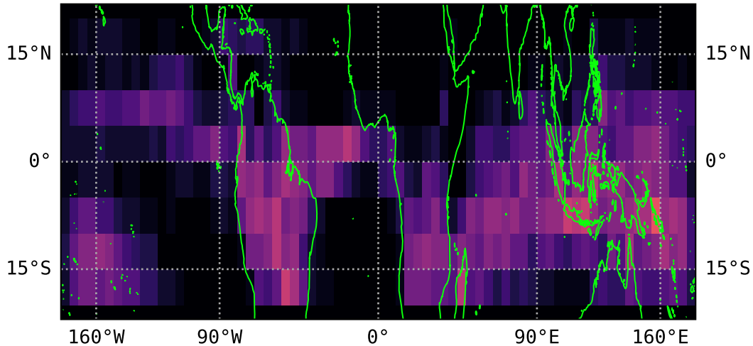
GPM PF PDF [%]
