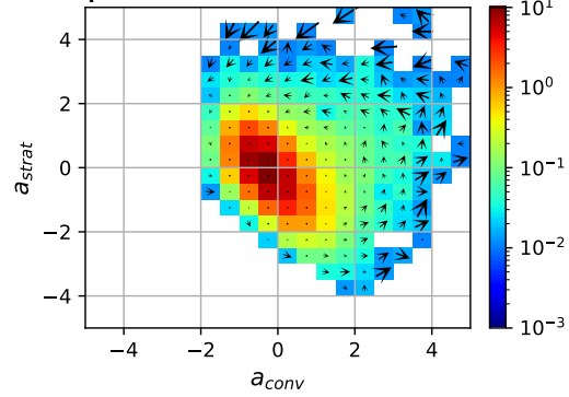
F ERA5 CENTERED
