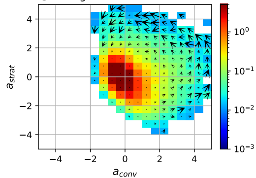
C gSAM CENTERED
