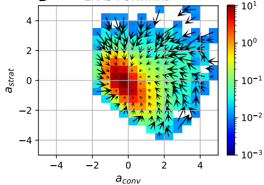
D ERA5 FORWARD
