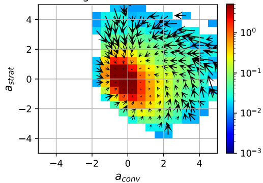
A gSAM FORWARD
