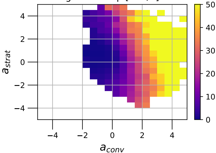
gSAM Precip [mm/d]
