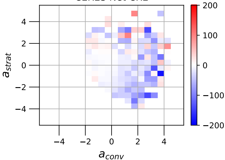
CERES Net CRE
