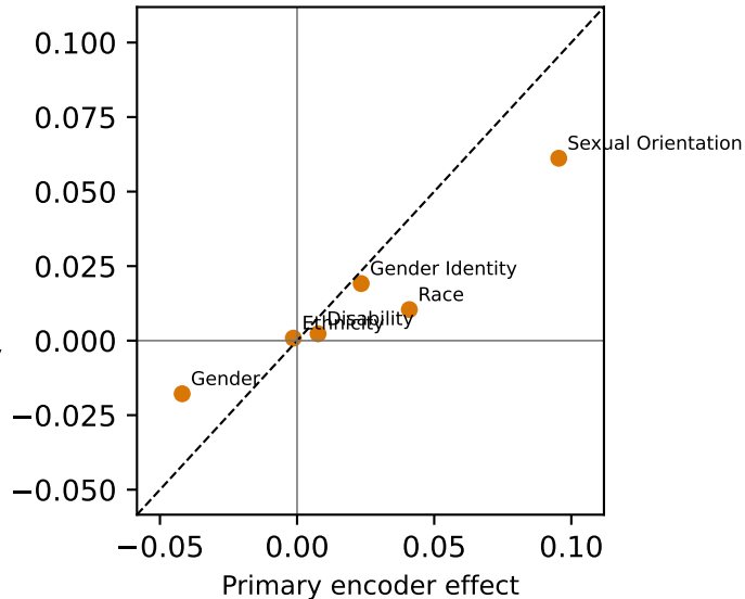
Evidence alignment
