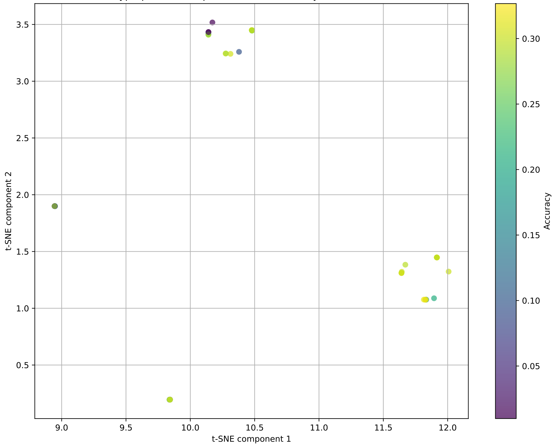
Hyperparameter Space Search for TwoLayerNet Modified
