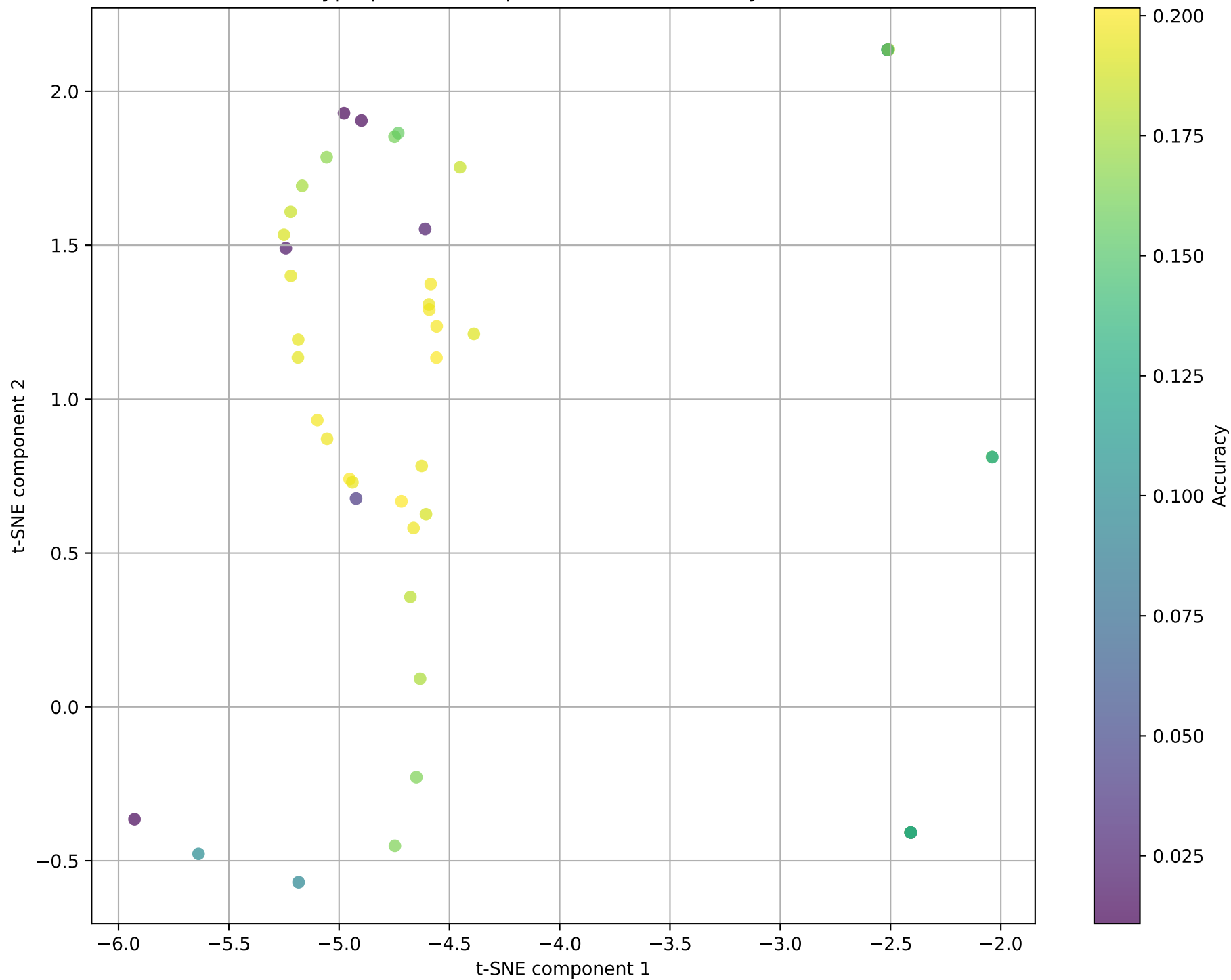
Hyperparameter Space Search for TwoLayerNet
