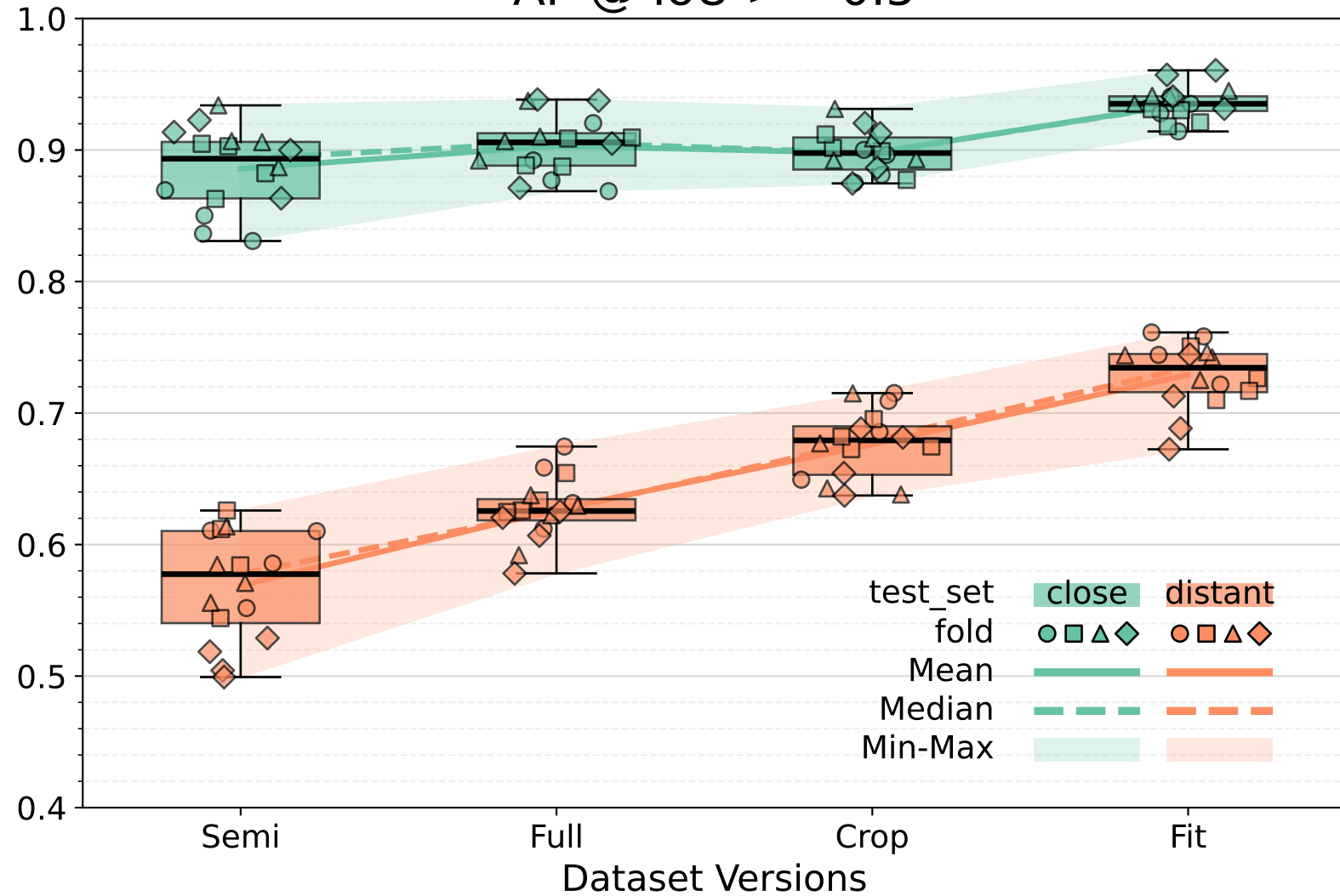
AP @ IoU \geq 0.5
