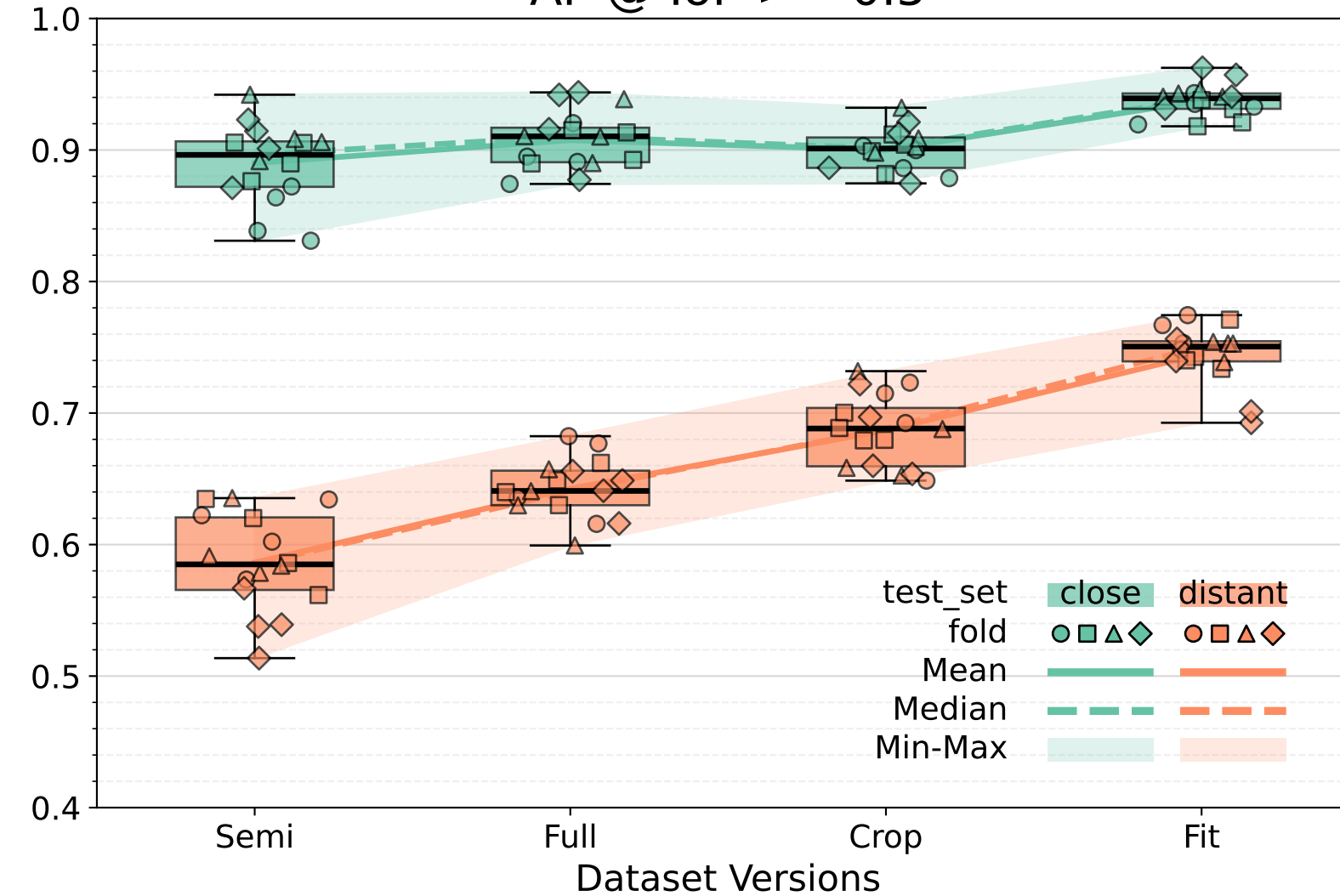
AP @ IoP \geq 0.5
