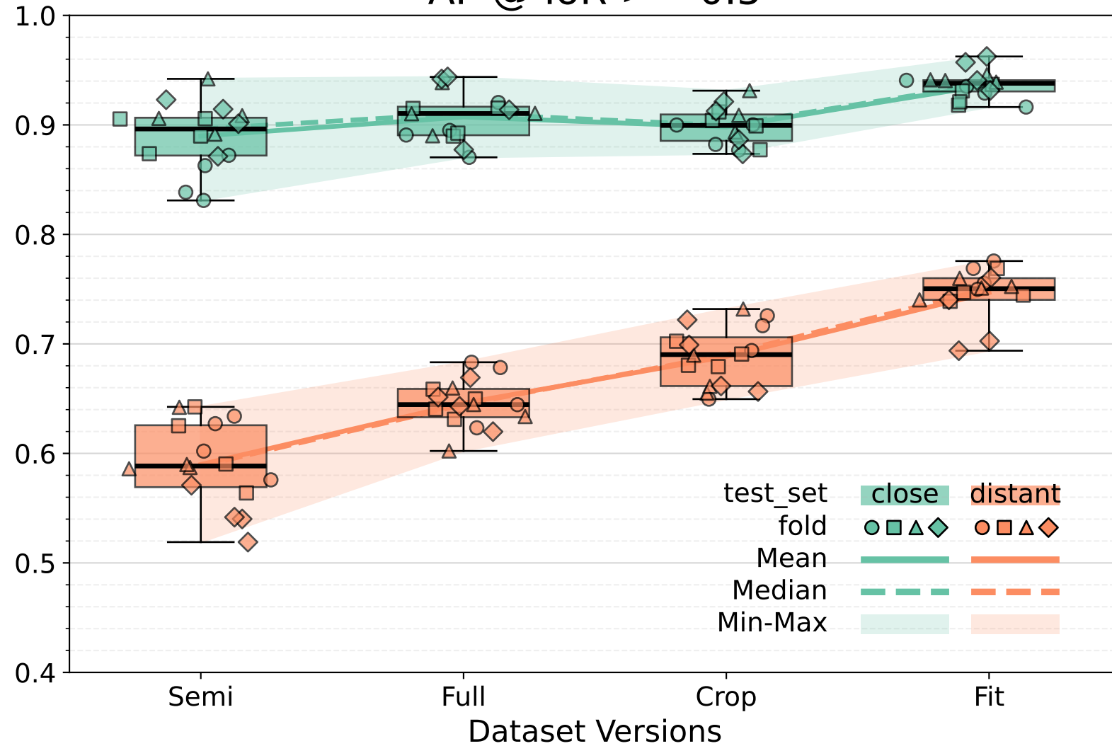
AP @ IoR \geq 0.5
