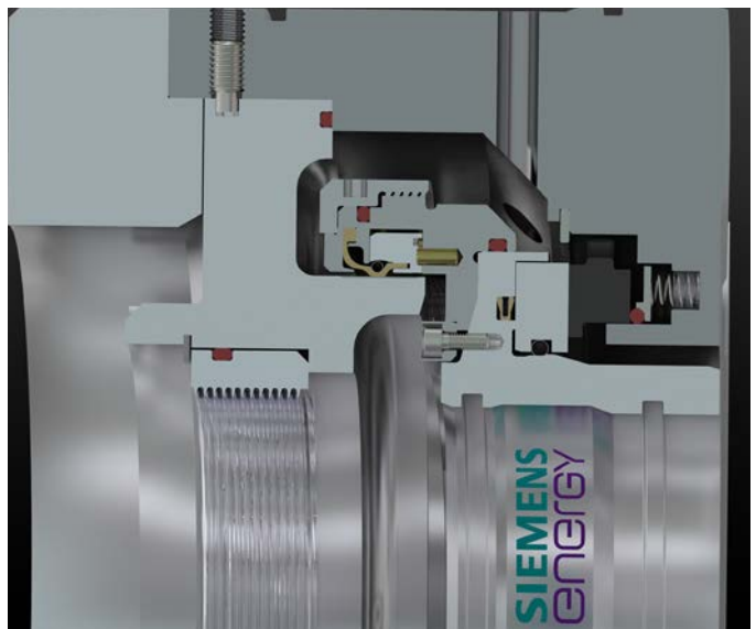
Seal Protect coupled with Siemens Energy dry gas seal system.
