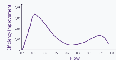
Figure 4: The diagram shows the turbine efficiency improvement at different flow rates after the optimization
