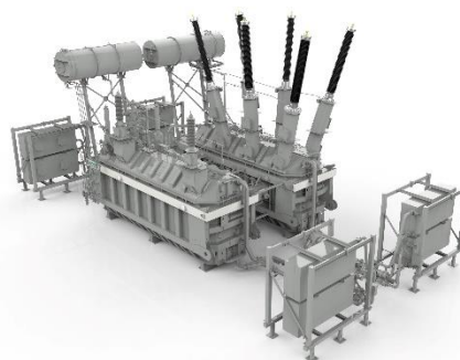
Standard phase-shifting transformer
