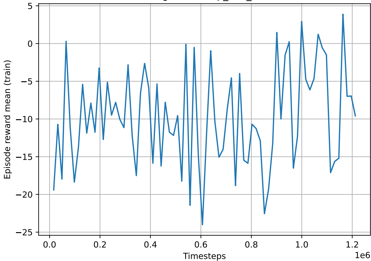
Training: rollout/ep_rew_mean
