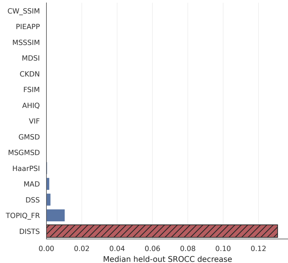
IQA blocks
