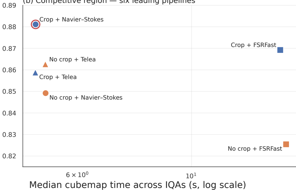
(b) Competitive region — six leading pipelines
