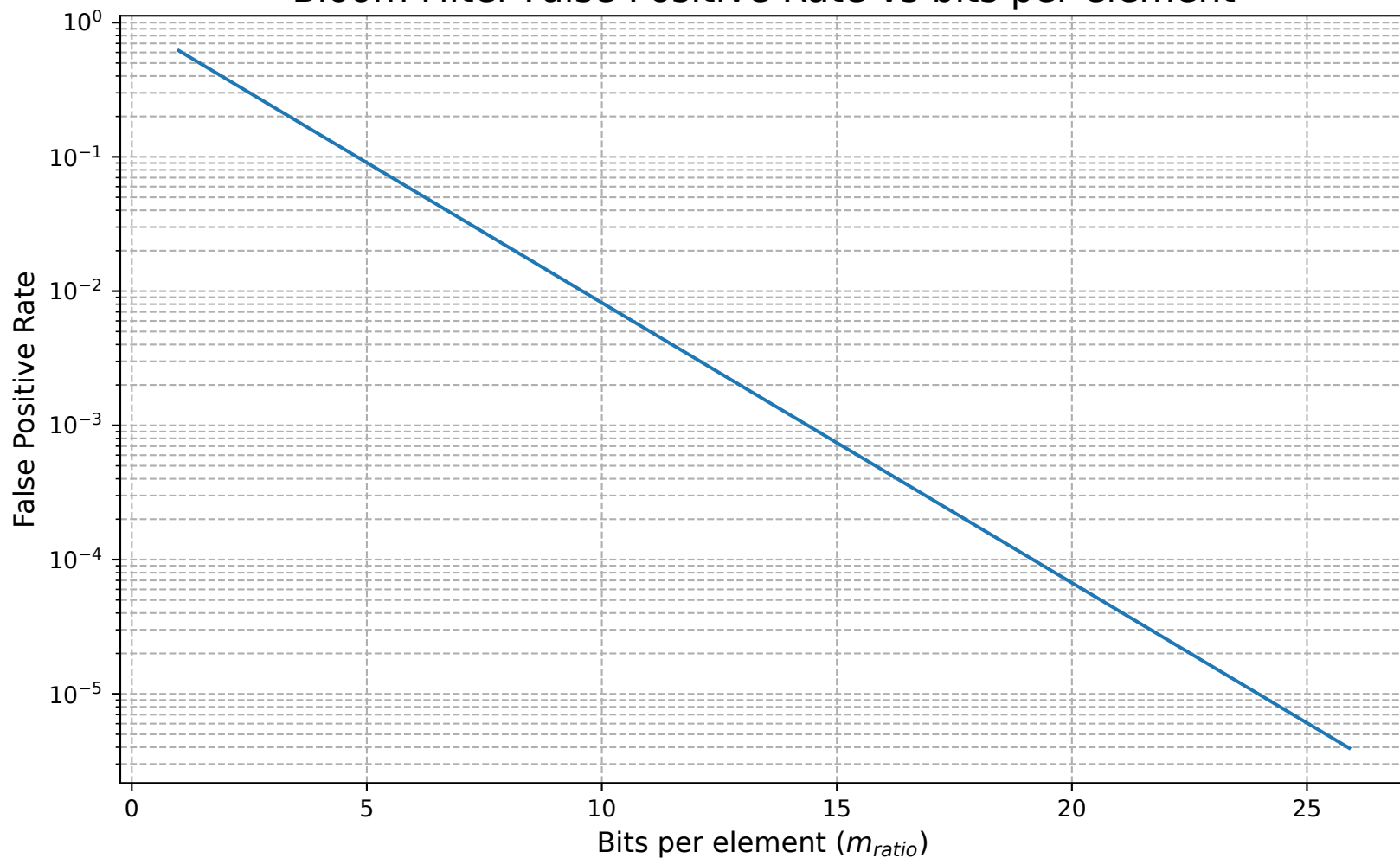
Bloom Filter False Positive Rate vs bits per element
