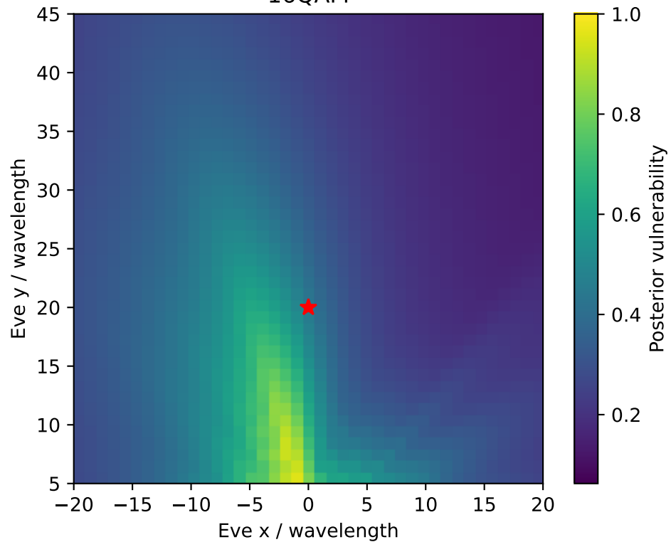
16QAM
