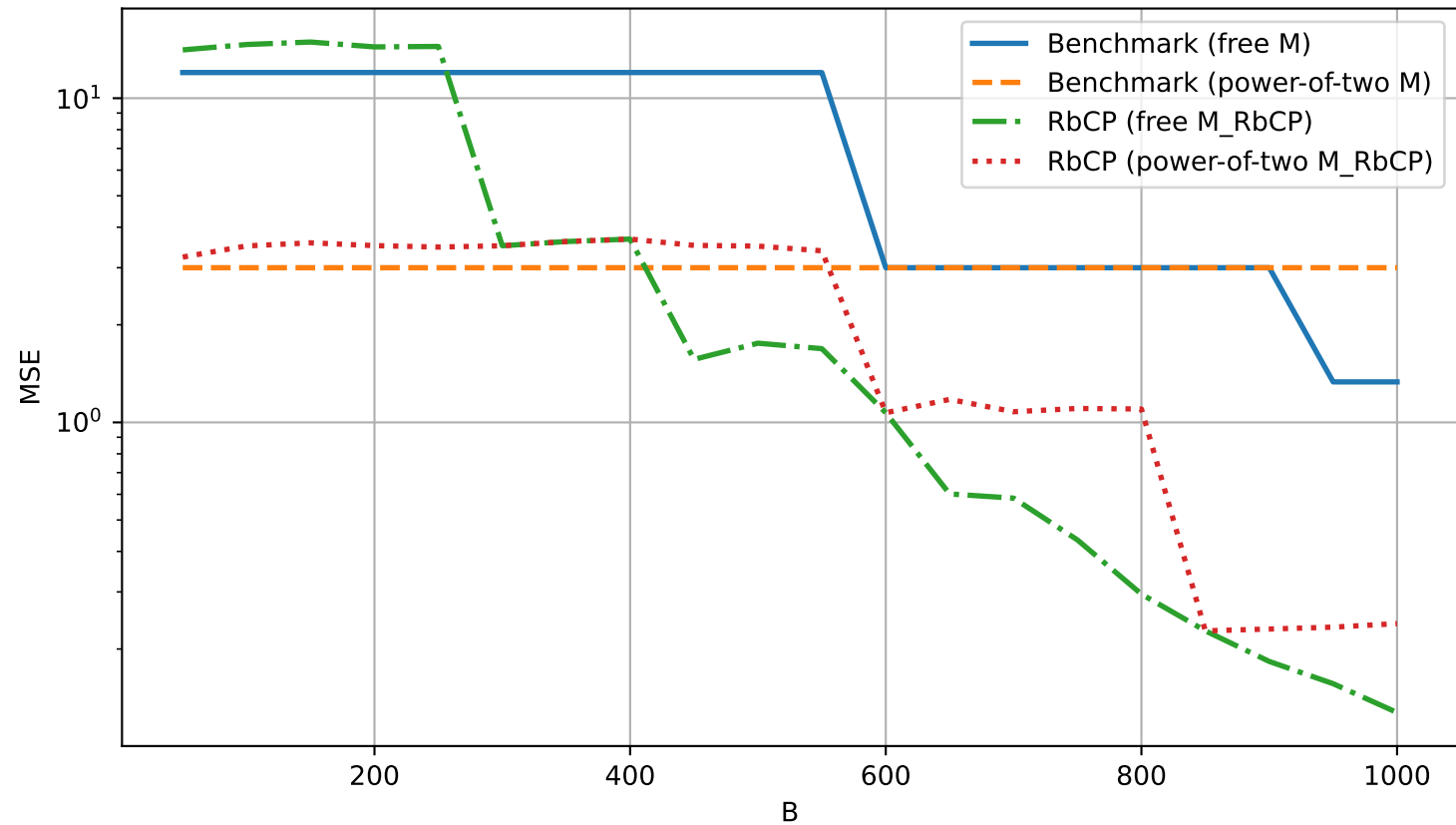
Benchmark and RbCP MSE versus B: free vs power-of-two truncation
