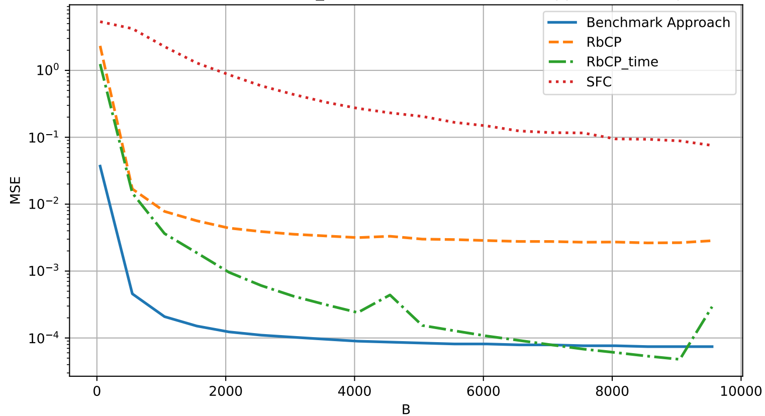
MSE versus B for RbCP, RbCP_time, SFC, and Benchmark Approach (fixed power)
