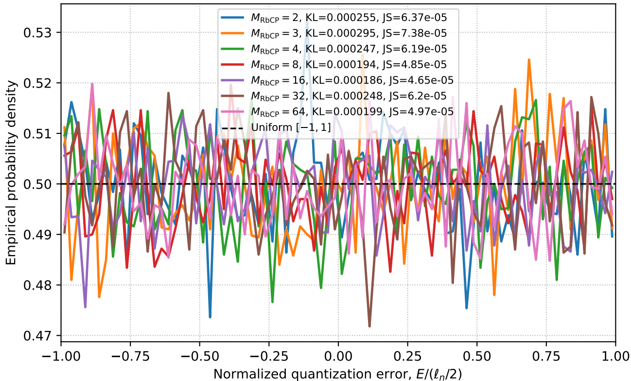
RbCP quantization error distribution: random_signal
