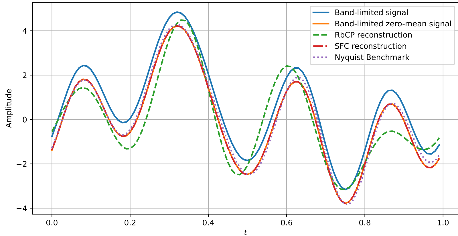
RbCP vs SFC vs Nyquist Benchmark
